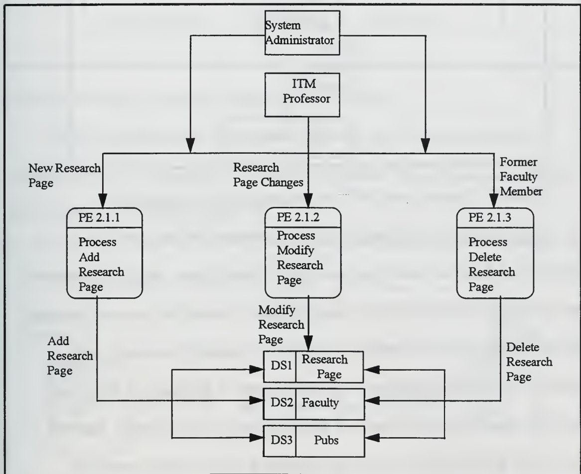
Figure 7. Primitive Level DFD For Maintaing a Research Page
